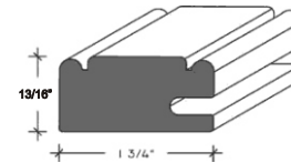
1 3/4" Drawer Front Profile
